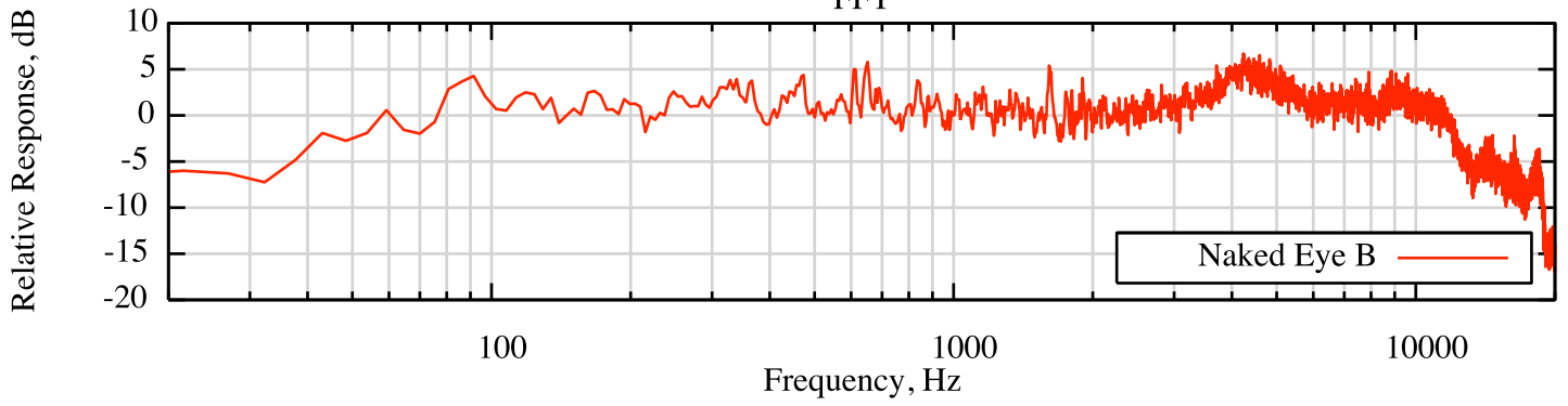
Exponential Moving Average
